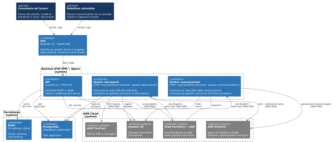
Figura 2: Container Diagram
